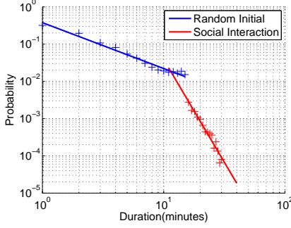
Fig. 2. Duration distribution
